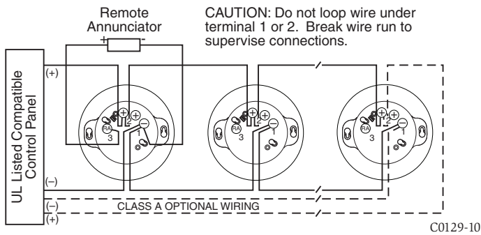
FIGURE 2. WIRING DIAGRAM
